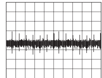
④ IC302 (13) (DVD play) 100 mV/DIV 50 ms/DIV
