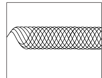
① IC302 (12) (CD play) 500 mV/DIV 200 ns/DIV
